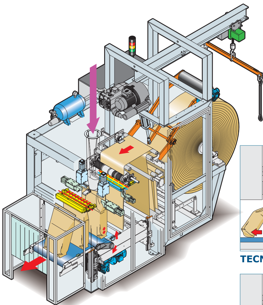
11 Evacuazione sacco pieno - Filled bag evacuation - Evacuation sac plein
