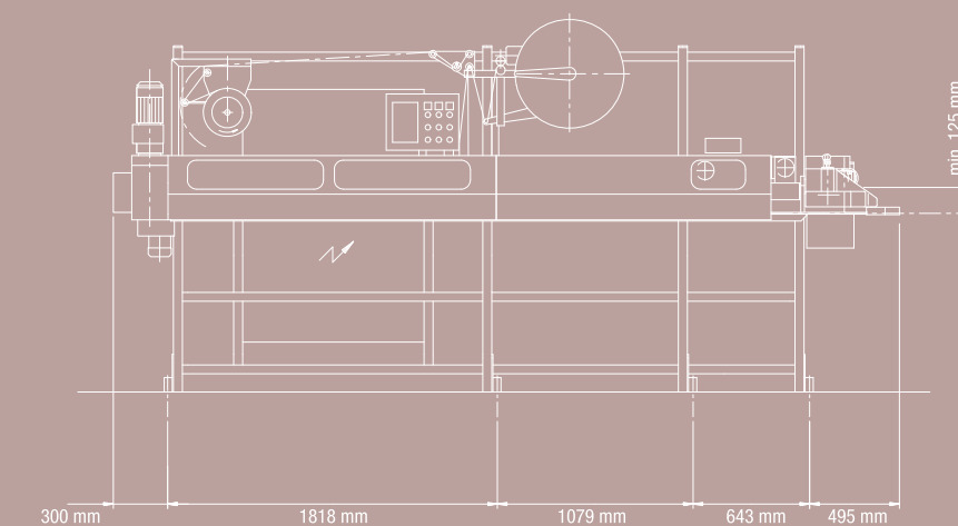
Side view of the machine type FTS
